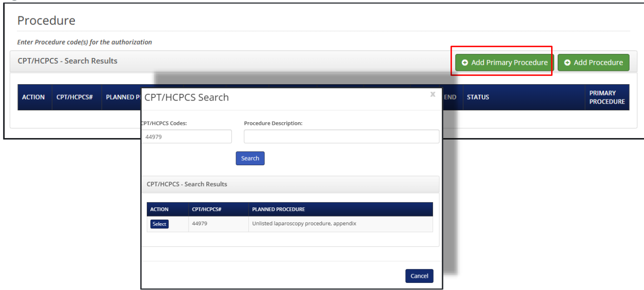
Figure 14: Procedure
