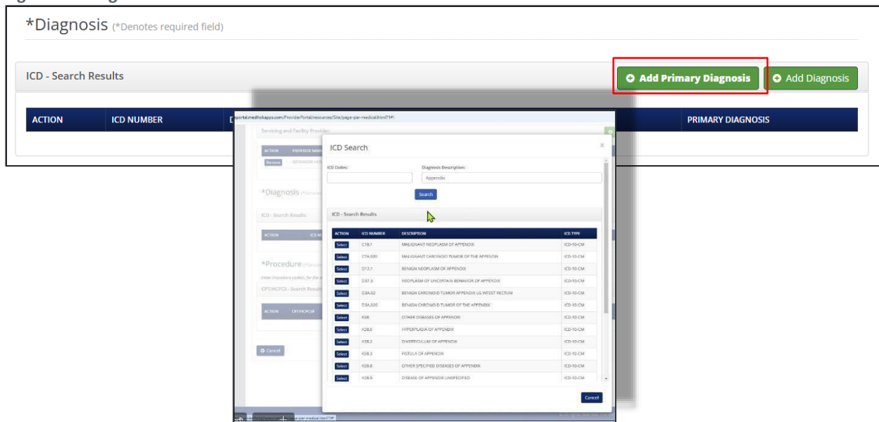
Figure 13: Diagnosis
