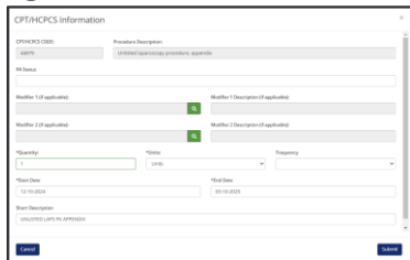
Figure 15: CPT/HCPCS Information
